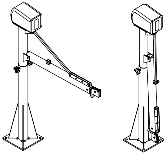
3D VIEW OF ASSEMBLED & COLLAPSED UNIT SHOWN FOR REFERENCE ONLY
